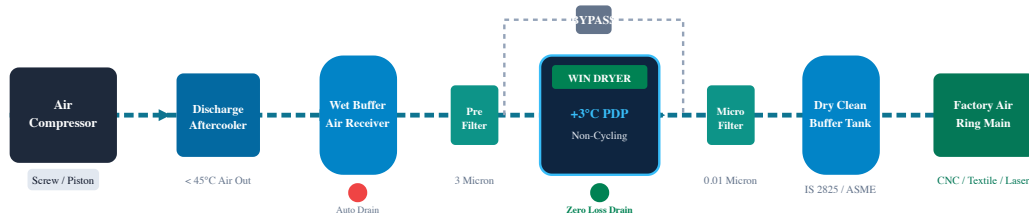
Figure 1: Standardized Win Equipments Compressor Room P&ID Flow Architecture
